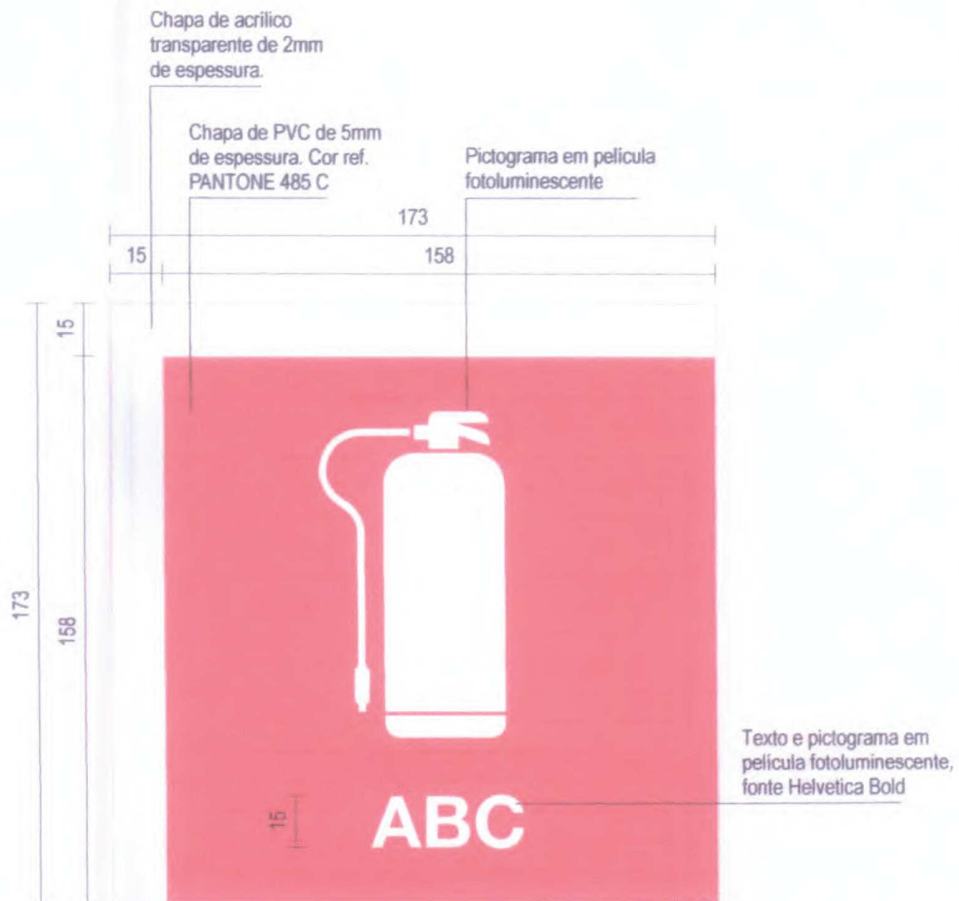
VISTA FRONTAL
